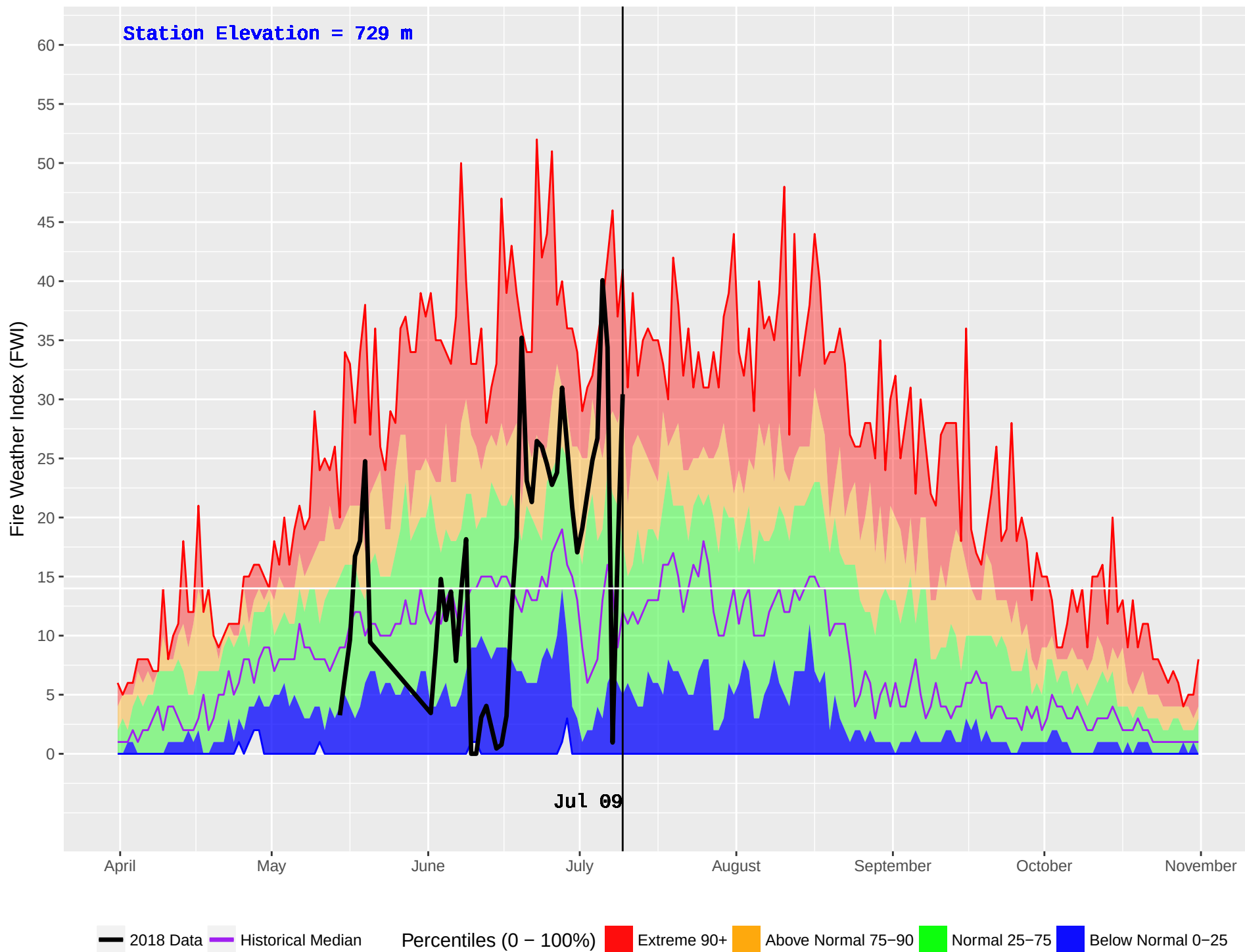
ATLIN (111) : Historical (1977–2016) and Current (2018) Daily Fire Weather Index (FWI)
