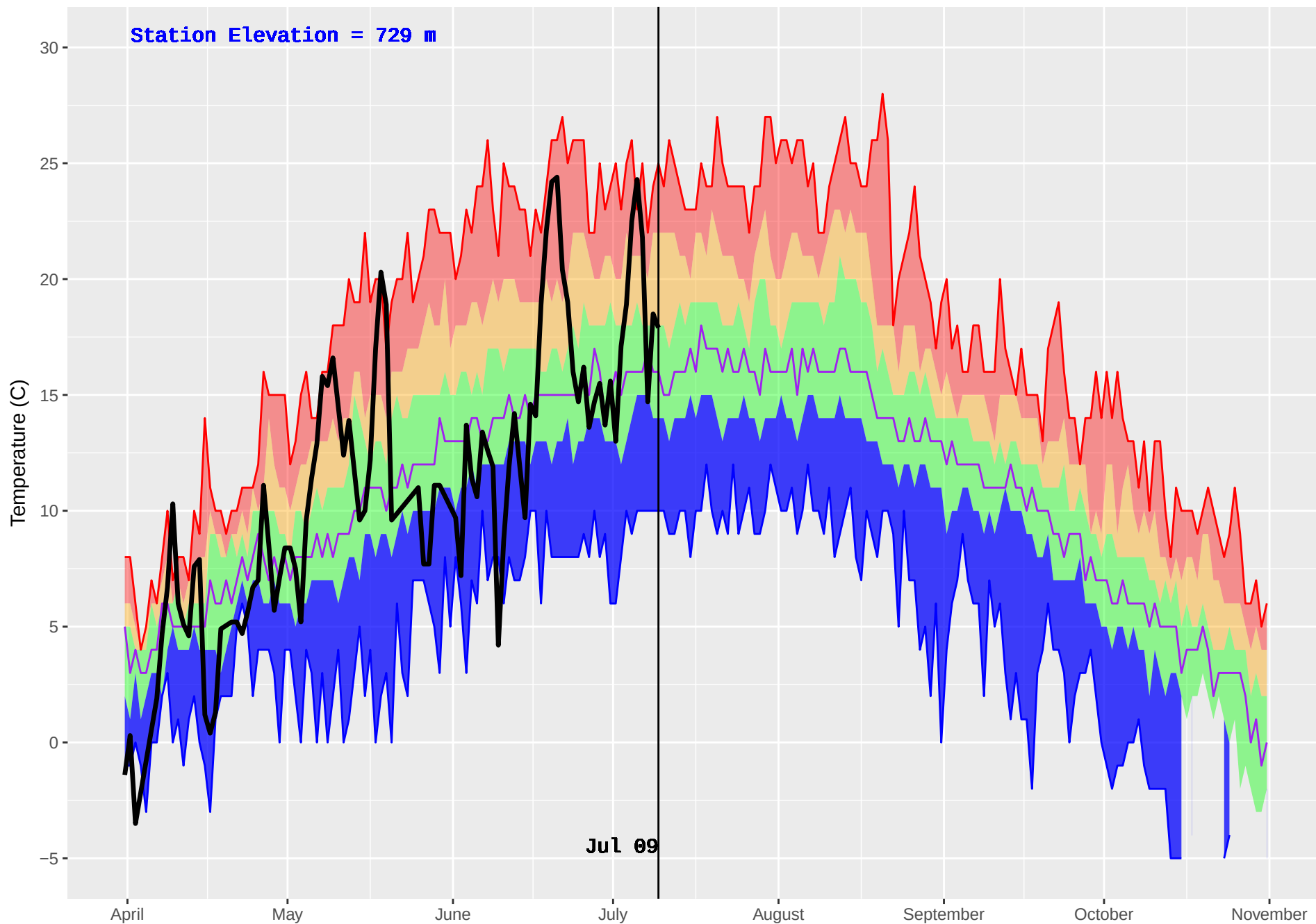
ATLIN (111) : Historical (1977–2016) and Current (2018) Daily Temperature
