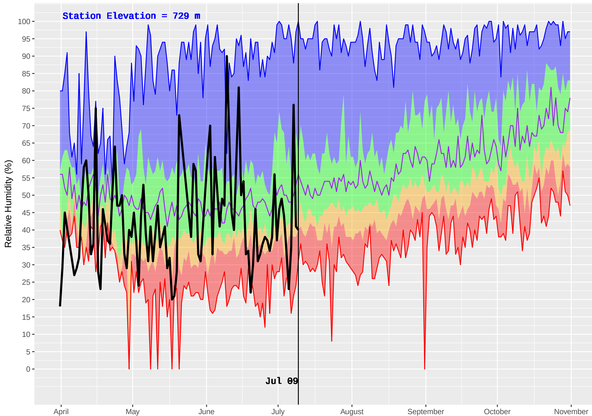
ATLIN (111) : Historical (1977–2016) and Current (2018) Daily Relative Humidity
