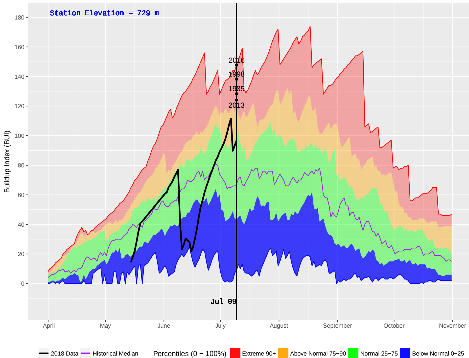
ATLIN (111) : Historical (1977–2016) and Current (2018) Daily Buildup Index (BUI)
