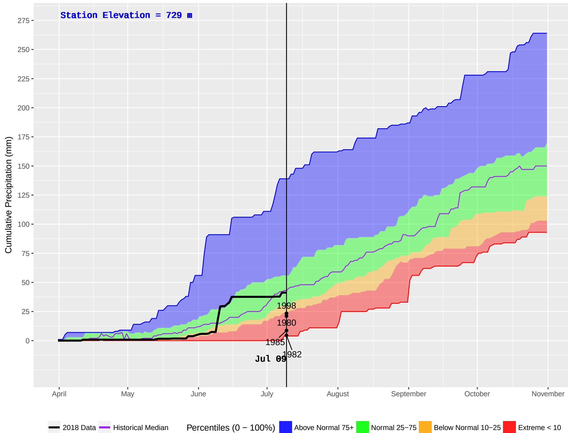
ATLIN (111) : Historical (1977–2016) and Current (2018) Daily Cumulative Precipitation
